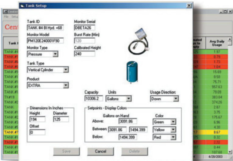
Typical tank setup from Centeron PC View Software
